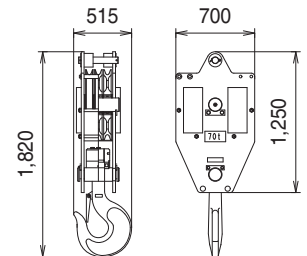
70 t Hook Weight: 900 kg
